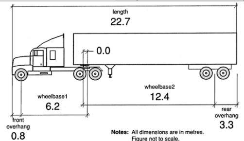
WB-20 Tractor-Semi-trailer Dimensions
