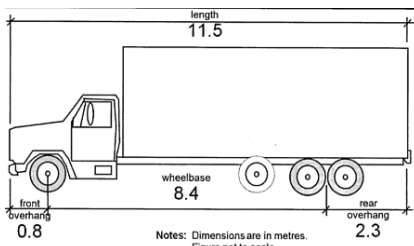
HSU Heavy Single Unit Truck Dimensions
